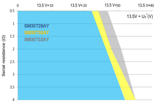
Figure 19. Load dump capability (typical values, U_S^* = f(R_i) pulse 5b, U_S = 87\text{ V} , t_p = 400\text{ ms} )
