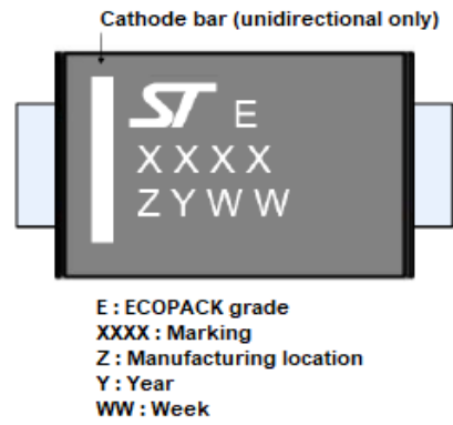
Figure 25. Marking layout
