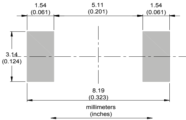
Figure 24. Footprint recommendation
