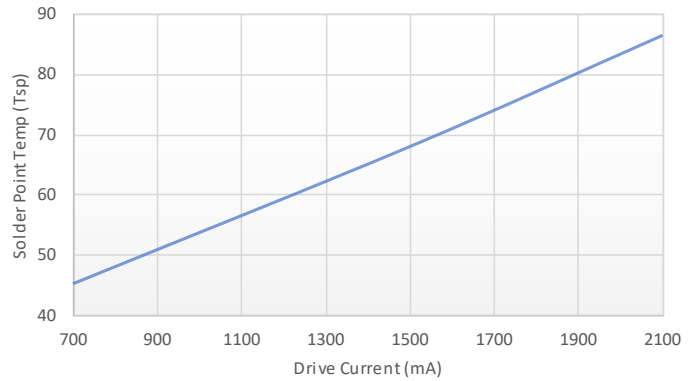
Tsp vs Drive Current
