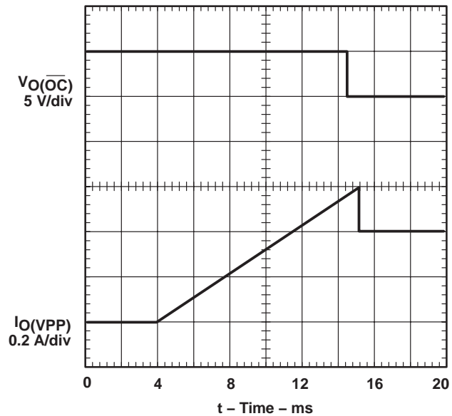
Figure 7. \overline{Vo(OC)} Response With Ramped Load on 12-V xVPP-Switch Output
