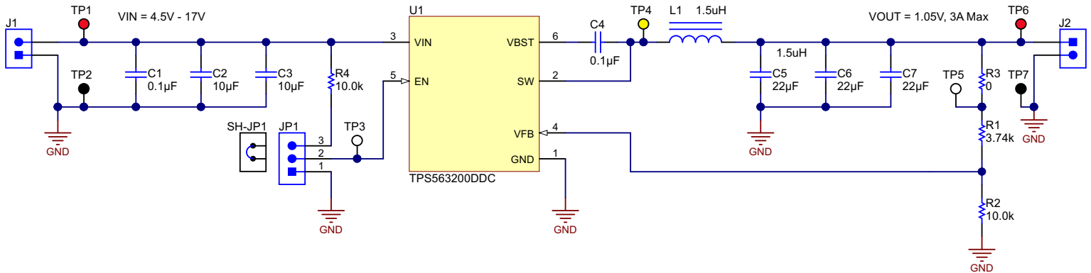
Figure 6-1. TPS563200EVM-652 Schematic Diagram
