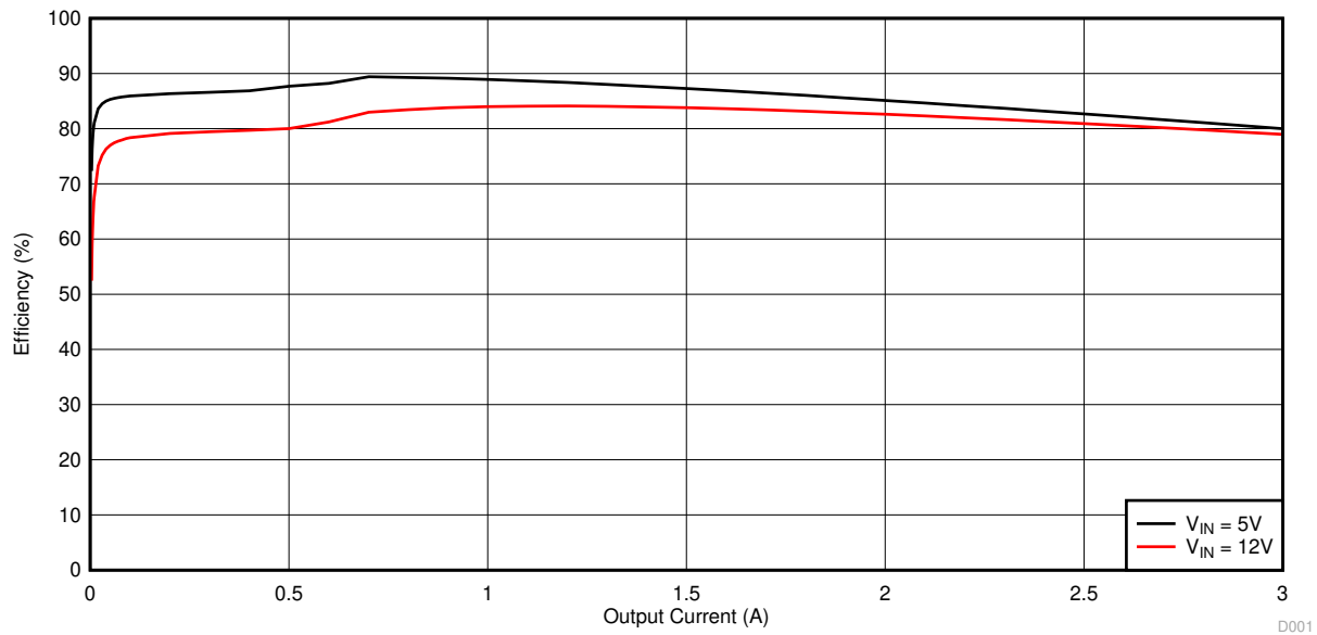
Figure 4-1. TPS563200EVM-652 Efficiency
