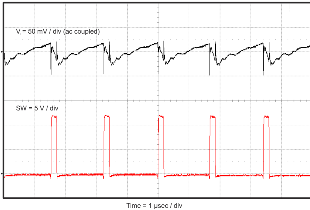
Figure 4-10. TPS563200EVM-652 Input Voltage Ripple, I_{OUT} = 3 A
