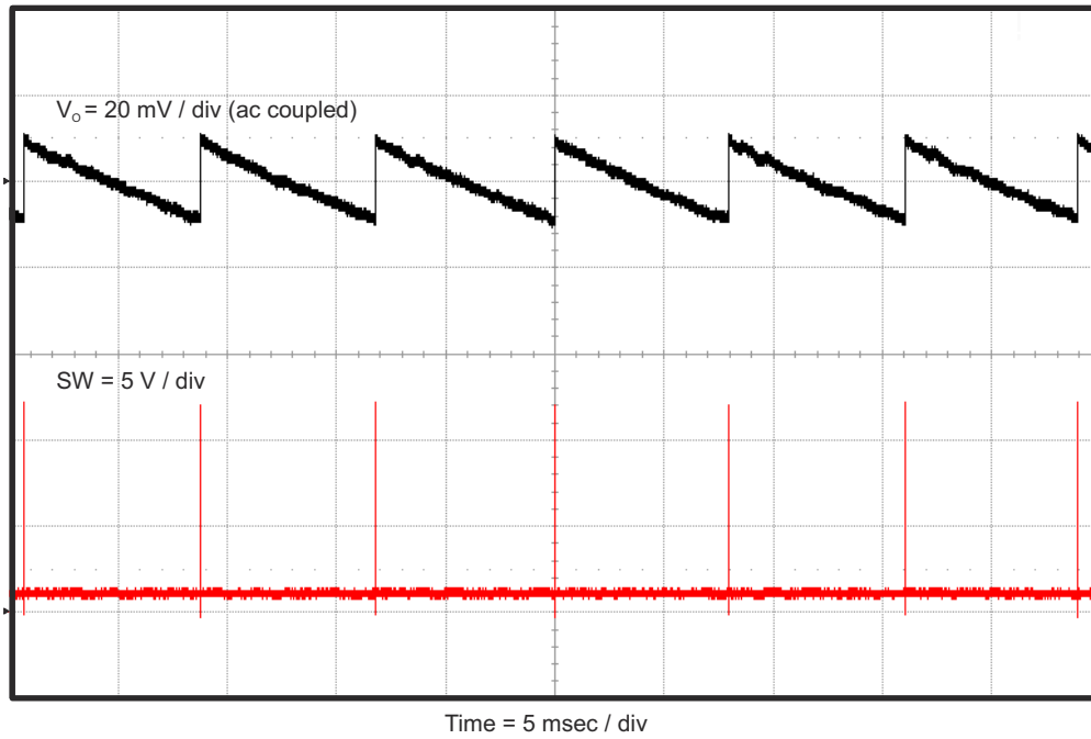
Figure 4-9. TPS563200EVM-652 Output Voltage Ripple, I_{OUT} = 0 mA
