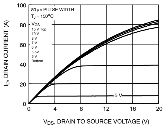
Figure 9. Saturation Characteristics
