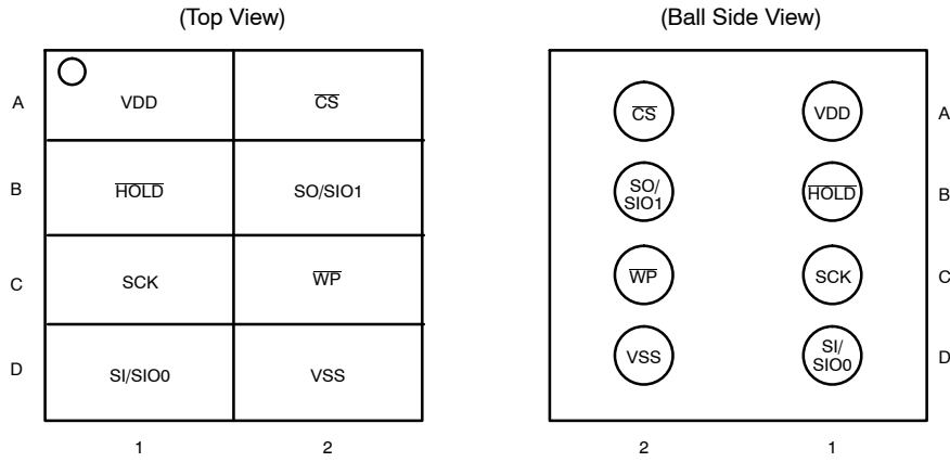
Figure 3. WLCSP8 (LE25S161XBTAG)
