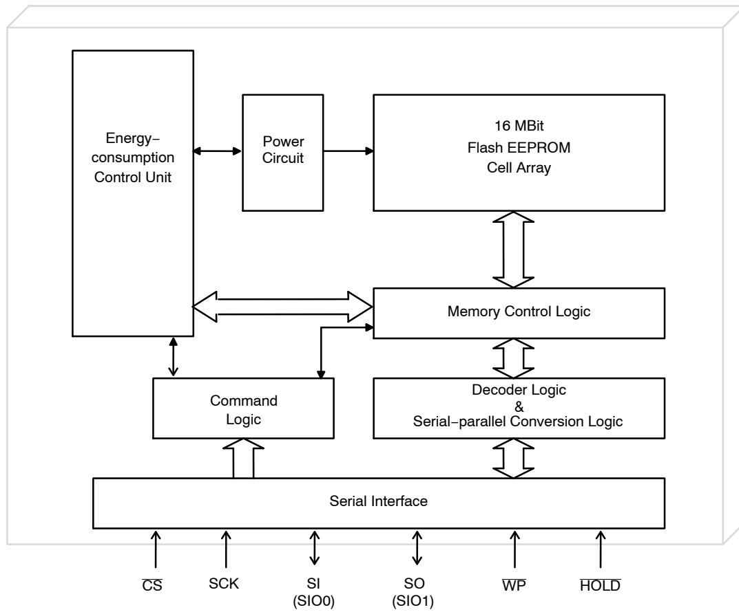
Figure 5. Block Diagram
